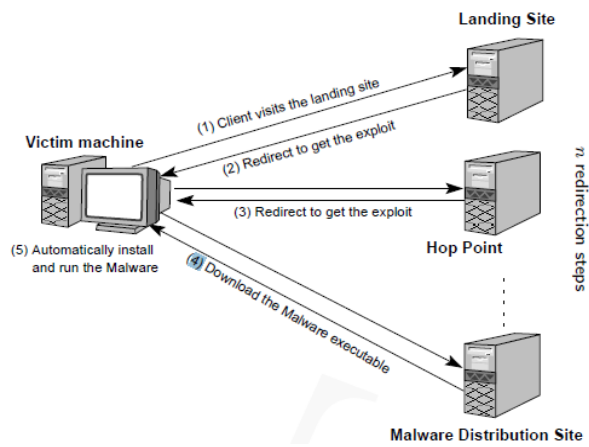
Fig. 2.1: A typical Interaction with of drive-by download victim with a landing URL.
